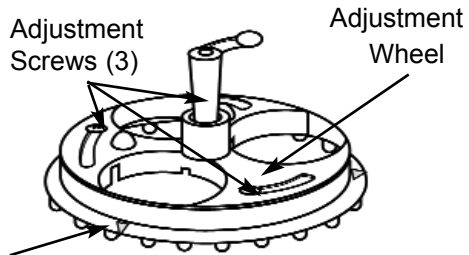
Wheel Alignment Arrow (align with center screw on coin mechanism)
